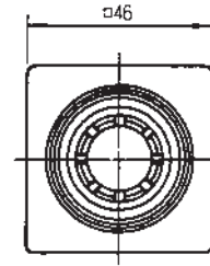
Mounting Cutout Model K402: 1.18" Dia. Model K4025: 1.00" Dia.
